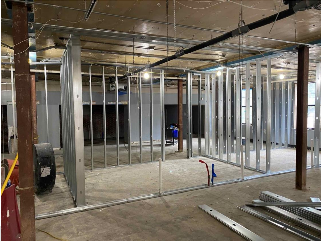
Interior framing at art/STEM room
